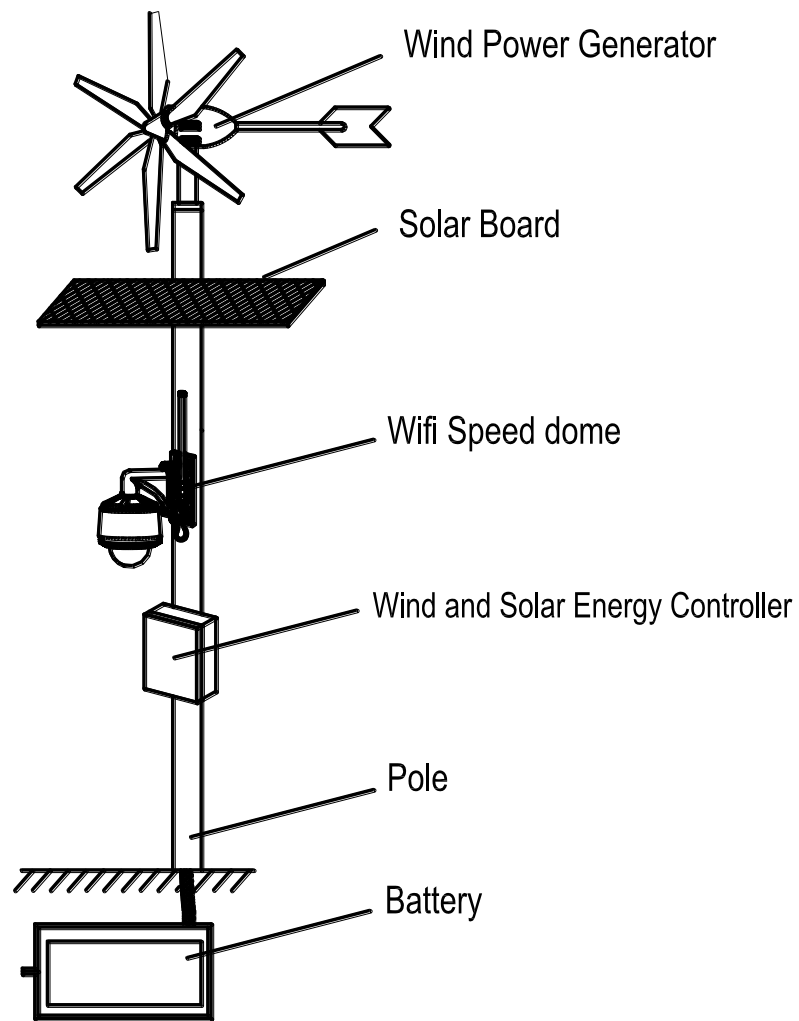
Installation Diagram
