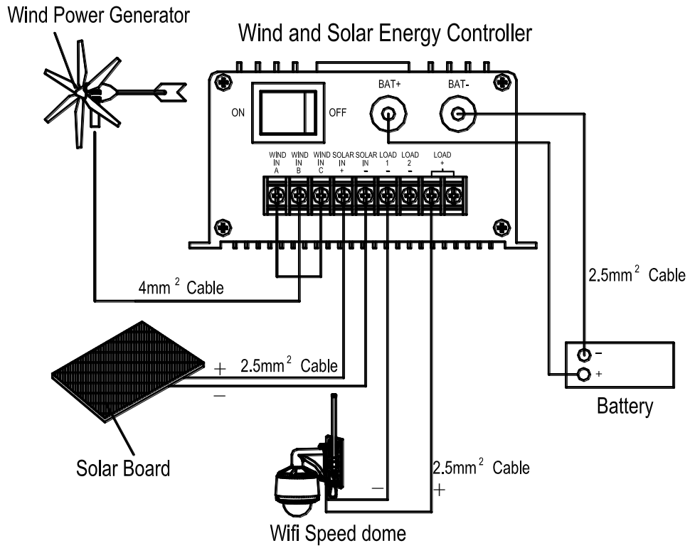
System connection diagram
